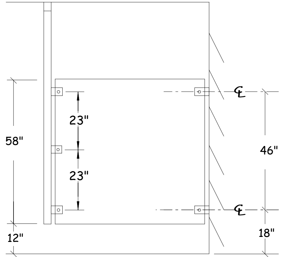
Series 50 - Typical elevation Backing points for other than masonry walls indicated
