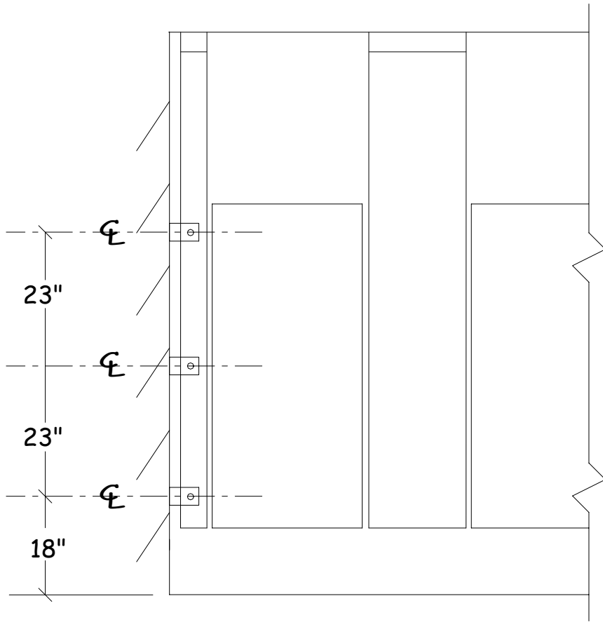
Series 50 - Typical elevation Backing points for other than masonry walls indicated
