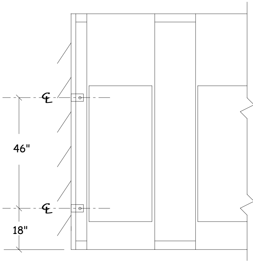
Series 60 - Typical elevation Backing points for other than masonry walls indicated
