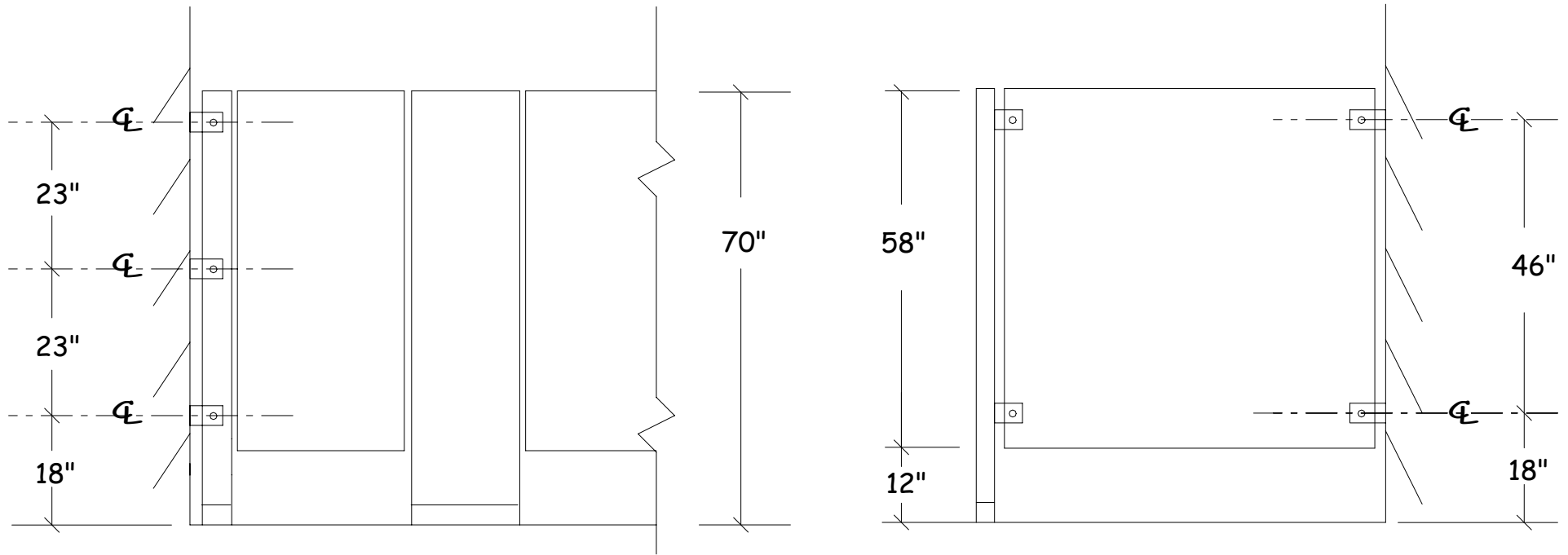
Series 30 - Typical elevation Backing points for other than masonry walls indicated
