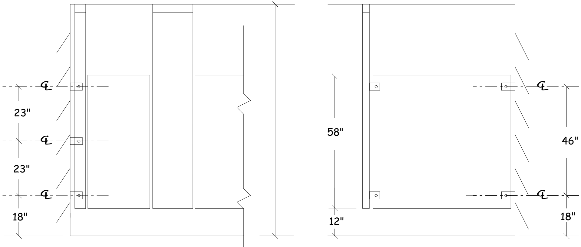
Series 50 - Typical elevation Backing points for other than masonry walls indicated
