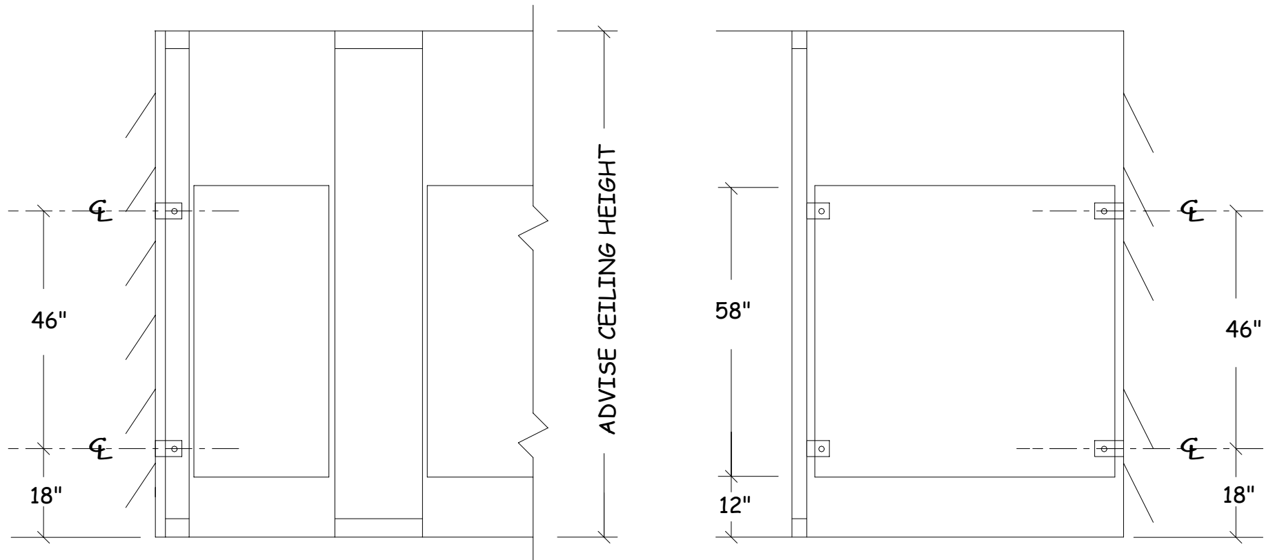
Series 60 - Typical elevation Backing points for other than masonry walls indicated
