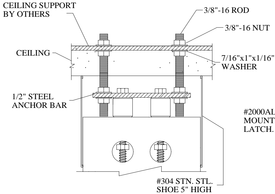
50-6 CEILING CONNECTION
