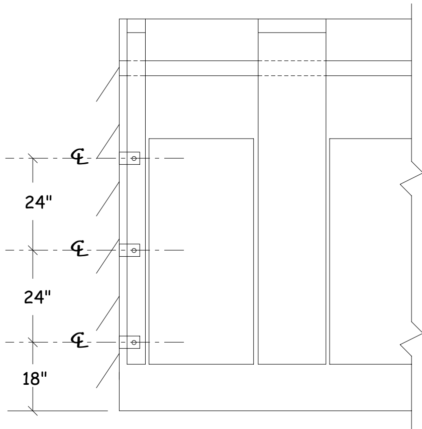
Series 50 - Typical elevation Backing points for other than masonry walls indicated
