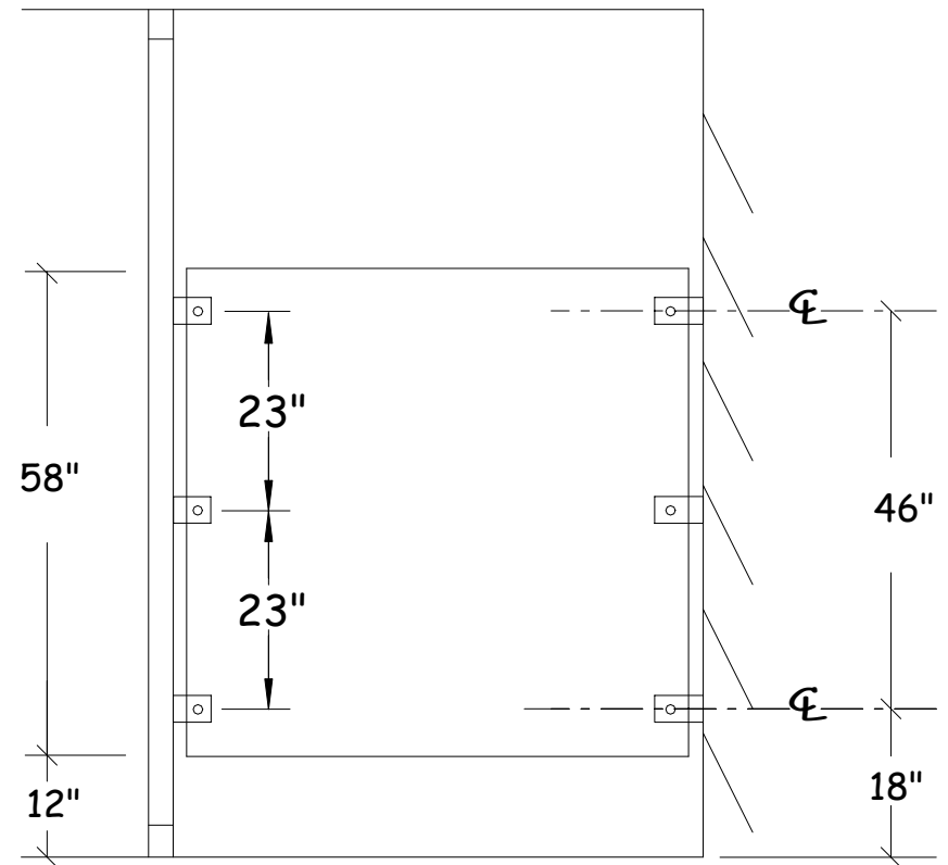
Series 60 - Typical elevation Backing points for other than masonry walls indicated
