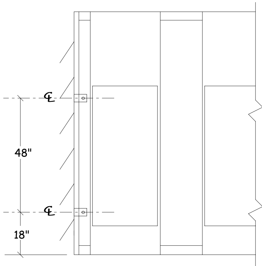
Series 60 - Typical elevation Backing points for other than masonry walls indicated
