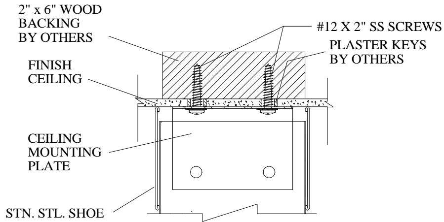
CEILING CONNECTION
