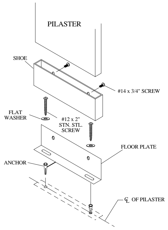
FLOOR CONNECTION
