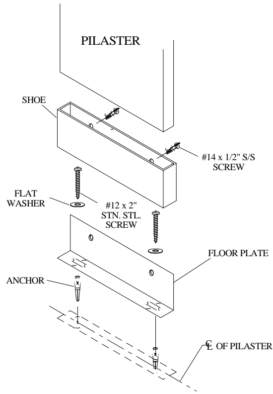
FLOOR CONNECTION
