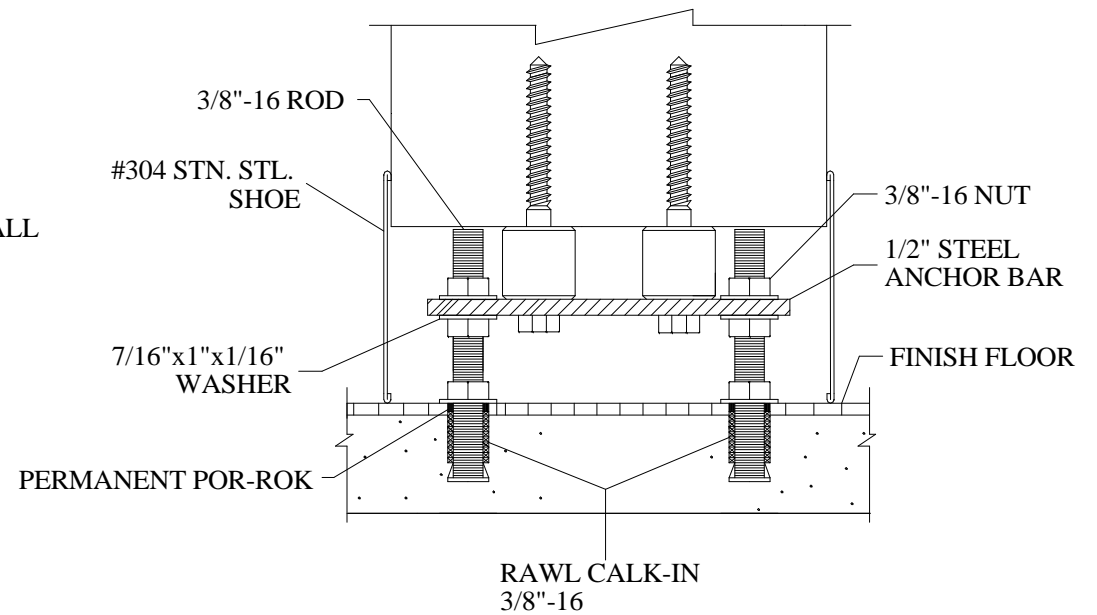
30-4 FLOOR CONNECTION
