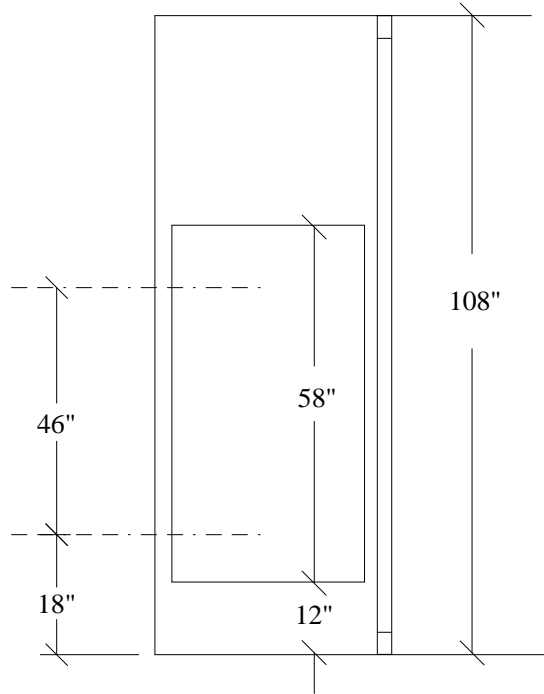
BACKING LOCATIONS
