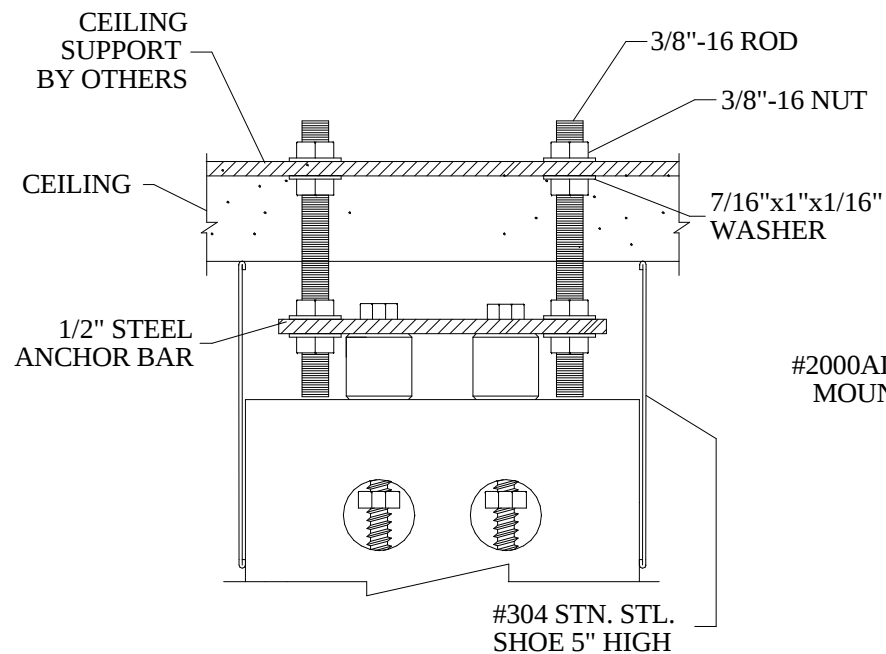
50-6 CEILING CONNECTION
