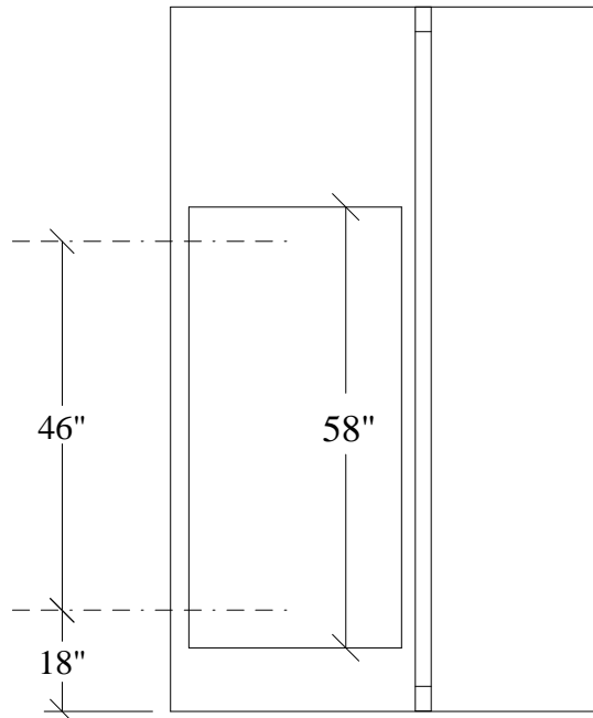
BACKING LOCATIONS
