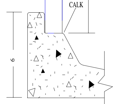
SECTION C-C
